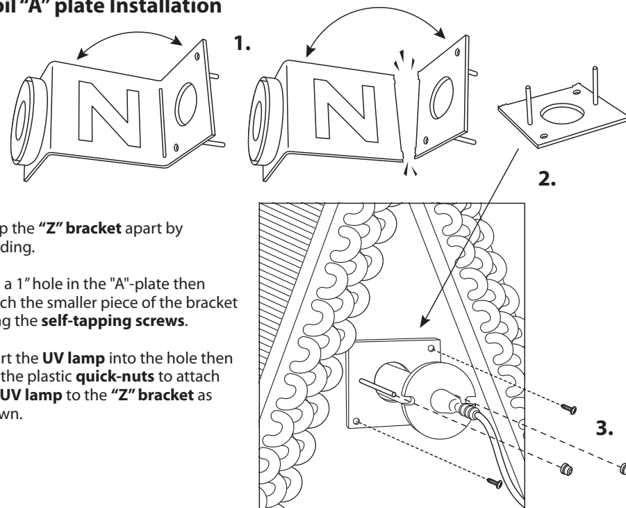
Blue-Tube UV® Mounting Options
