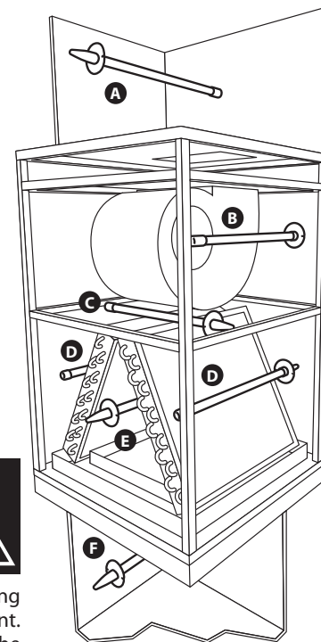
Blue-Tube UV® Mounting Options
